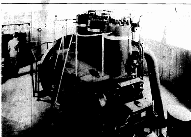
USES DIESEL POWER—Generating power for the 25 kw. transmitter of KSTP, St. Paul, is this 250 hp. Diesel engine. The engine drives a 135 kw. generator, which generates a 440-volt alternating current. Considerable economy of operation is reported by the station, which claims to be the only American broadcaster using Diesel power.
